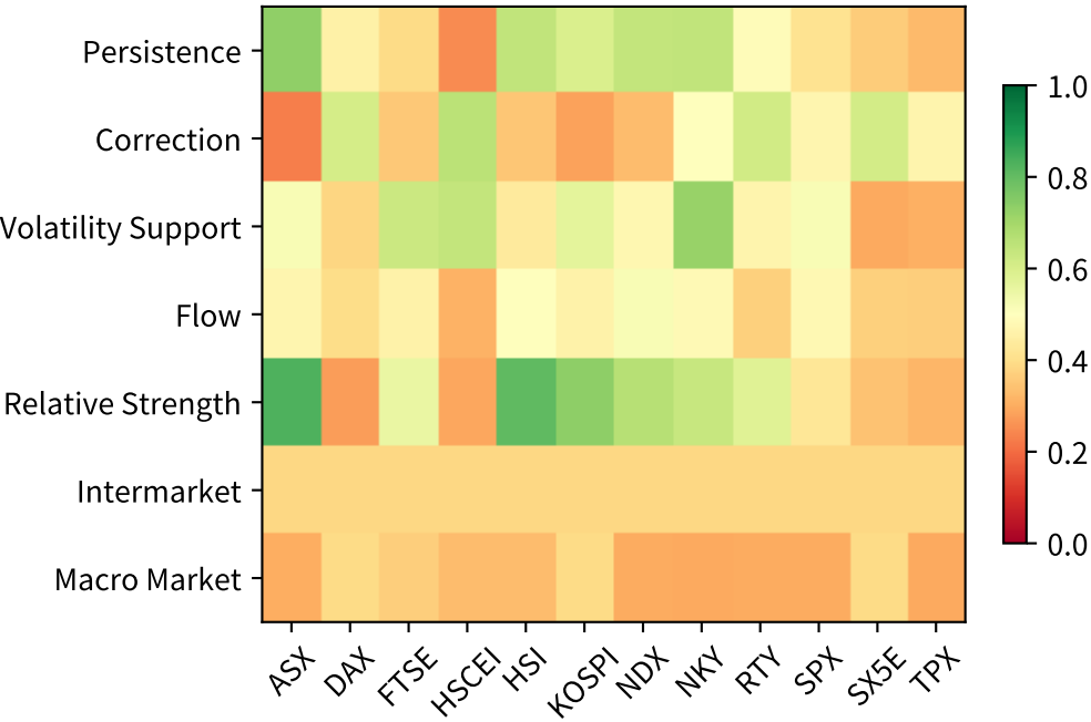
Evidence-only composite score
