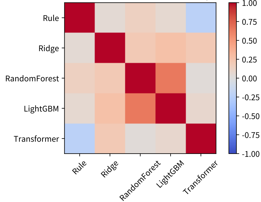
Prediction correlation / diversity
