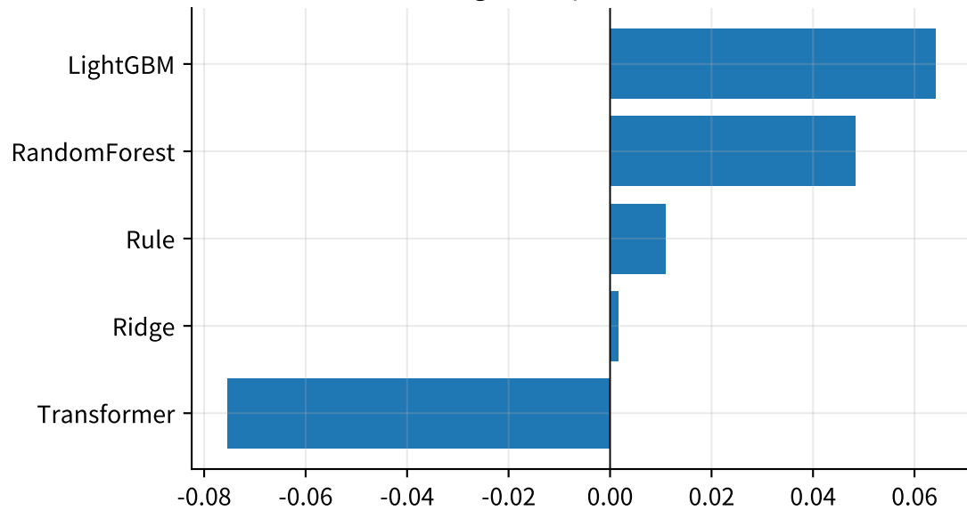
Average test-period Rank IC
